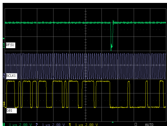
Figure 8: Timing Diagram 1
