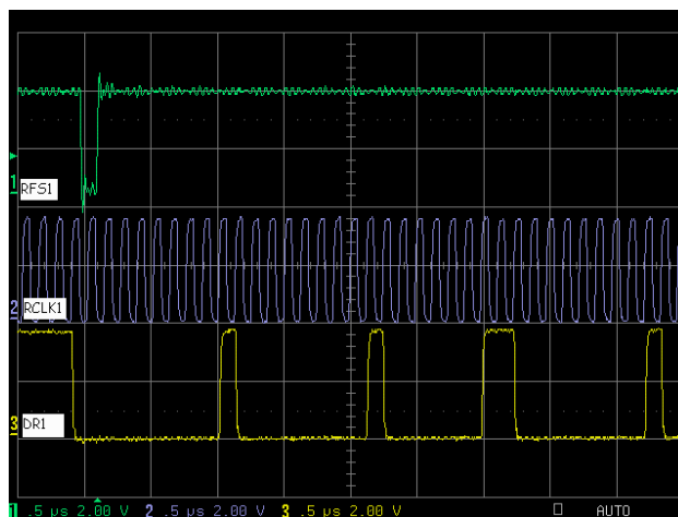
Figure 9: Timing Diagram 2
